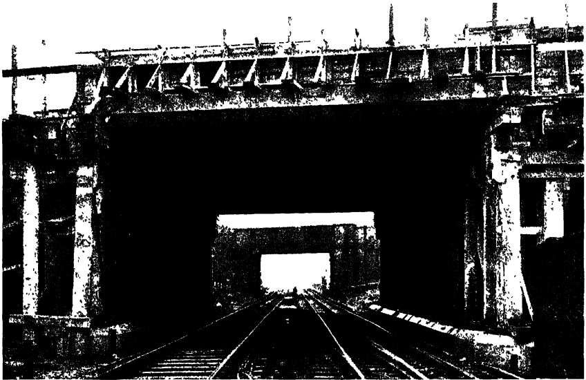
Fig. 302.—Shuttering for Bridge with Restricted Headroom.
